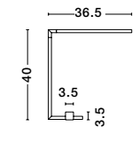
RACCIO - 9180725 Brass Gold Metal & Acrylic LED 6.8 Watt 230 Volt 280Lm 3000K IP20 L: 36.5 W: 12 H: 40 cm
