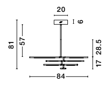
RACCIO - 9180781 Dimmable Brass Gold Metal & Acrylic LED 40 Watt 230 Volt 2800Lm 3000K IP20 L: 84 W: 80 H: 81 cm
