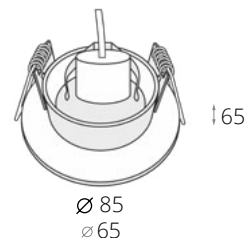
DL027-2-01B 1xGU10 50W H: 65, D: 85 mm, 220-240 V, IP20, Class 2
