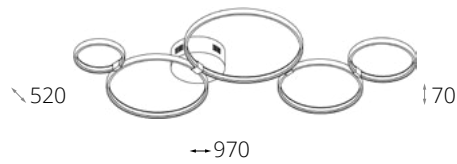
▲ MOD448-55-N LED 45W H: 70, W: 970, L: 520 mm, 2000 Lumen, 3000 K, 80 RA, 120 °, 220-240 V, IP20, Class 2
