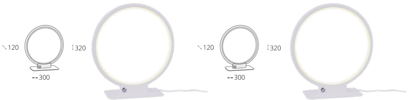
▲ MOD877TL-L18W ☞ LED 18W H: 320, W: 300, L: 120 mm, 900 Lumen, 3000 K, 80 RA, 120 °, 220-240 V, IP20, Class 2, Dimmable
