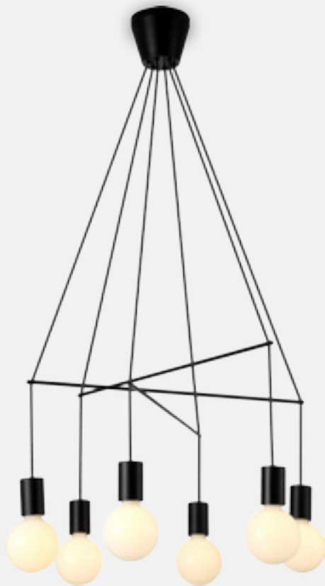
17200 TWIG metal-matt black 6xE27/G95/40W/ ↔670mm ↕1000mm EAN 8585032235368
