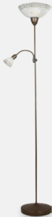
879 POMPEZ metal-brown gold / glass-alabaster decor 1x E14/40W/1xE27/100W / ↔280mm ⚡1755mm EAN 8586007086862
