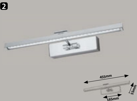
1 3640 M • LED / 5W (300lm, 3000K) incl. IP20 chrome
