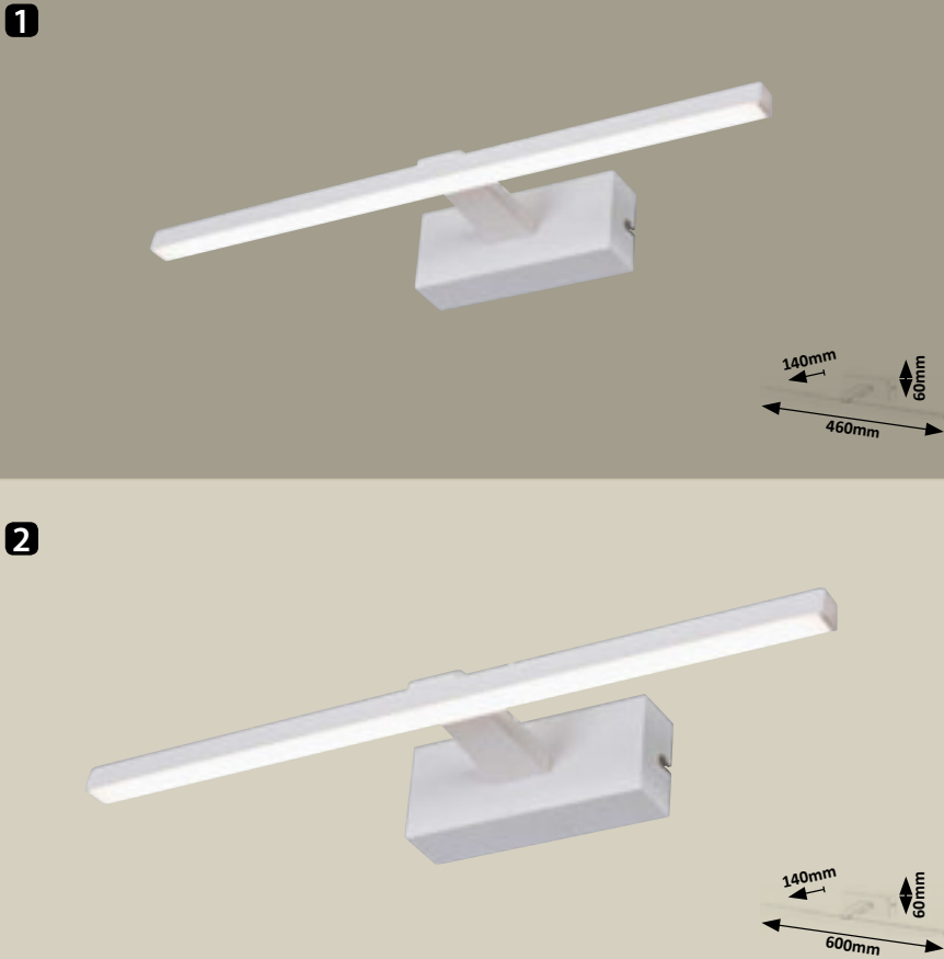
1 I448 M P • LED / 8W (450lm, 4000K) incl. IP23 matte white
