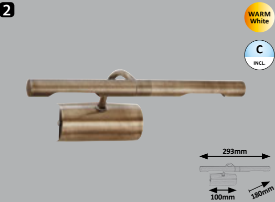
1 3643 M • 28W (370lm, 2700K) incl. G9 / 2x max. 40W • IP20 satin chrome 5 998250 336435 2 3644 M • 28W (370lm, 2700K) incl. G9 / 2x max. 40W • IP20 bronze 5 998250 336442 3 3641 M E-14 / T25 / 2x max. 40W IP20 • satin chrome 5 998250 336411 4 3642 M E-14 / T25 / 2x max. 40W IP20 • bronze 5 998250 336428 Picture slim 1 3907 M • LED / 8W (316lm, 4000K) incl. IP20 chrome 5 998250 339078 2 3908 M • LED / 12W (466lm, 4000K) incl. IP20 chrome 5 998250 339085 3 3909 M • LED / 8W (321lm, 4000K) incl. IP20 chrome 5 998250 339092 4 3910 M • LED / 12W (554lm, 4000K) incl. IP20 chrome 5 998250 339108 rabalux 407
